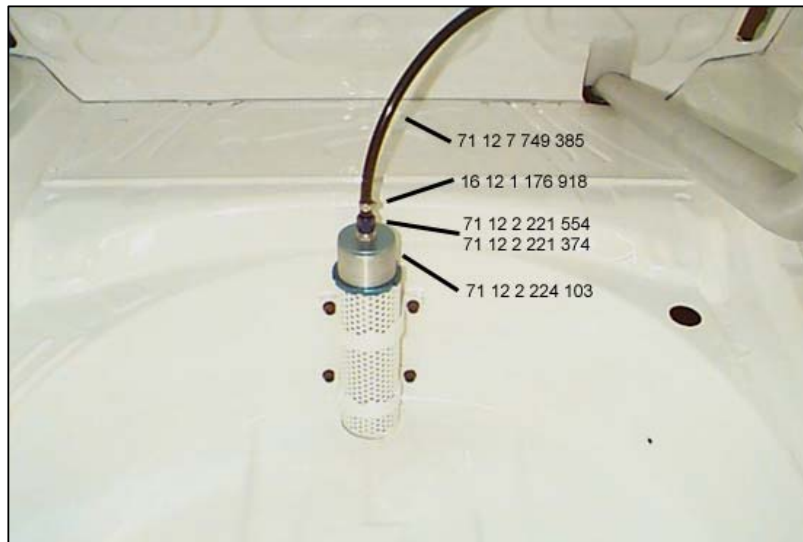
Wagenheber Fußraum rechts / air jack in passenger compartment front rh
